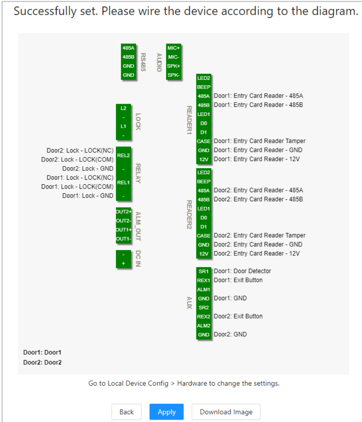
Figure 2-8 Wiring diagram
